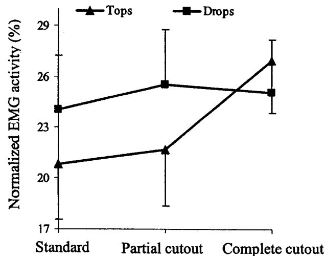
FIGURE 3—Normalized EMG activity values (mean, SEM, N = 20) for the standard, partial cutout, and complete cutout saddle conditions while participants rode with their hands on the tops and drops of the handlebars. A significant saddle design by hand position interaction
